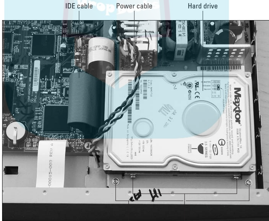
Figure 12-3: Examine TiVo to locate its hard drive, drive bay, IDE cable, power cable, and anything else listed in your kit's instructions.
